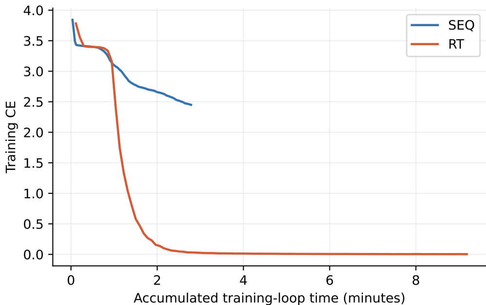
A5 training · nonoverlapping 100-update means Time excludes evaluation, checkpointing and W&B logging
