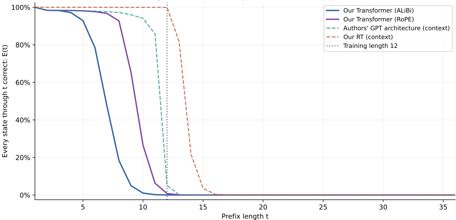
Figure 10-style cumulative accuracy · every curve at 50k E(t) only; solid lines are the paired ALiBi/RoPE comparison
