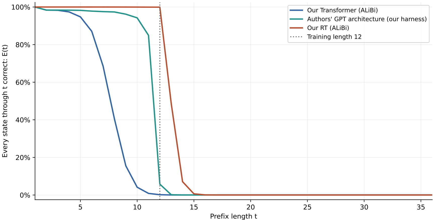
Figure 10-style cumulative accuracy · our fixed 100k experiment E(t) only; our results, not a digitization or reproduction of the paper
