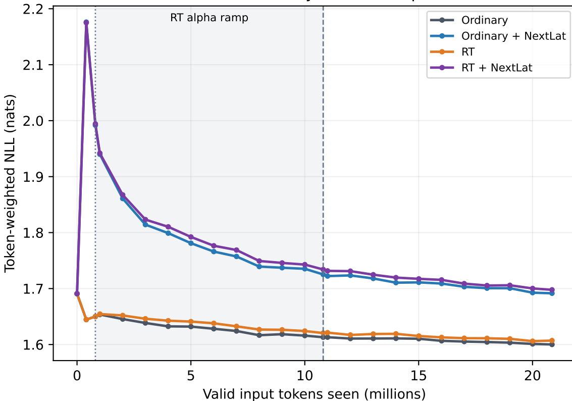
CodeSearchNet Python development
