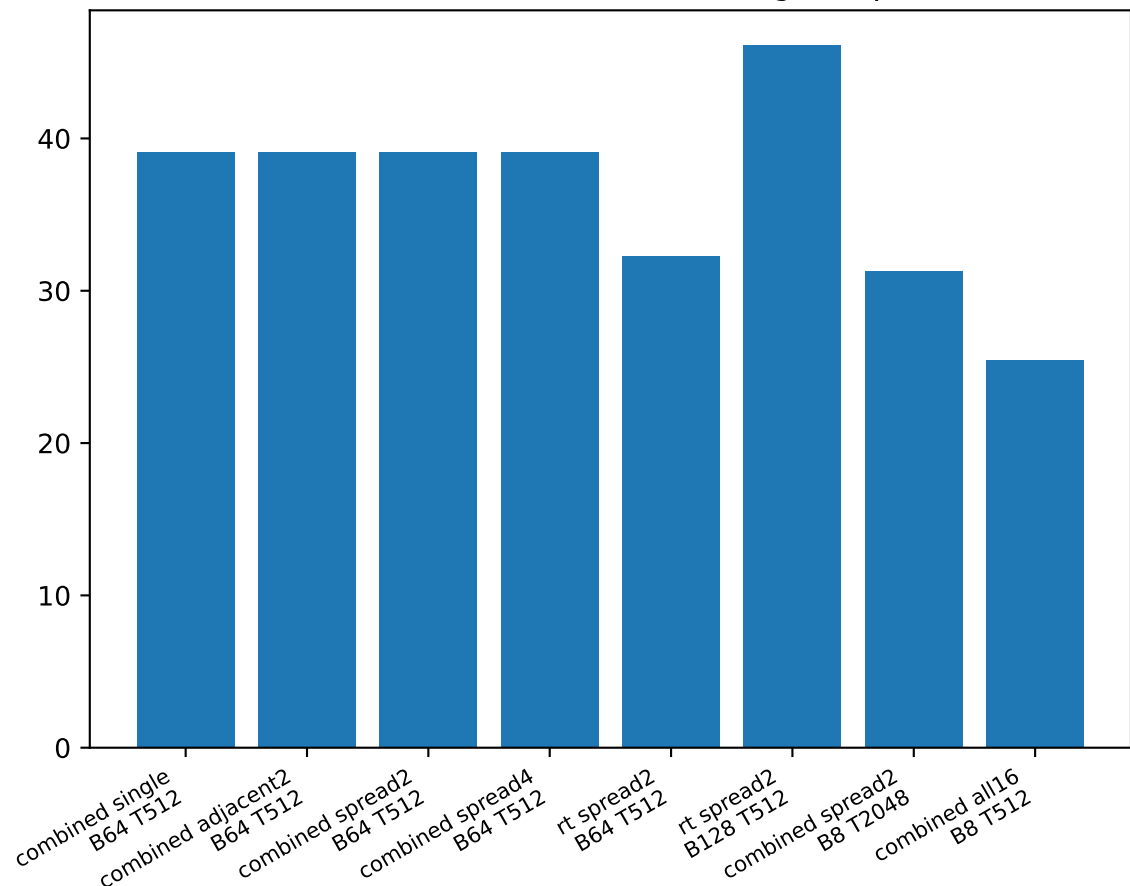
Peak allocated GiB, including setup
