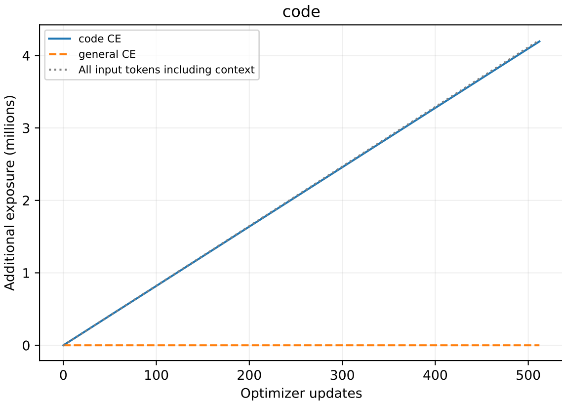
Matched CE budgets; unequal domain allocation and segment-context overhead
