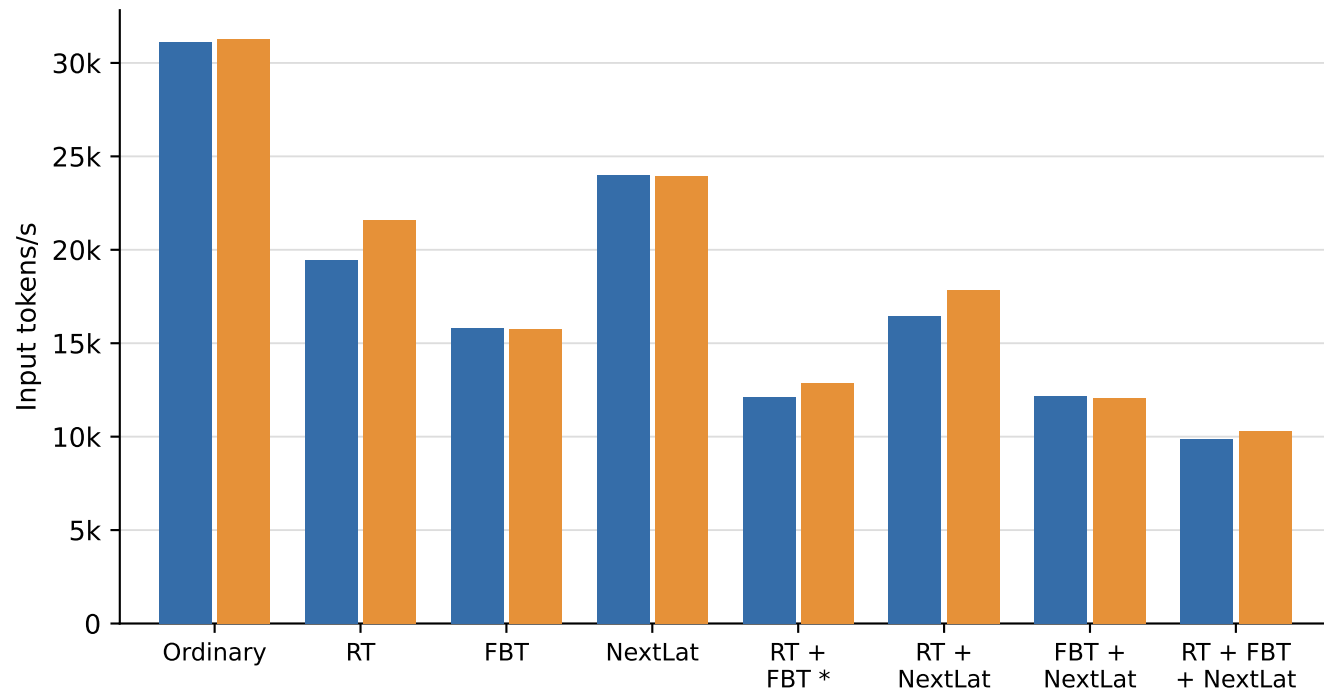
Full-update throughput
