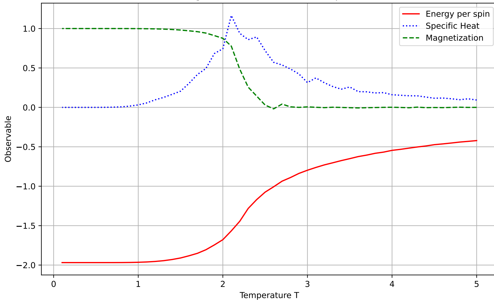
2D Ising Model Observables vs Temperature
