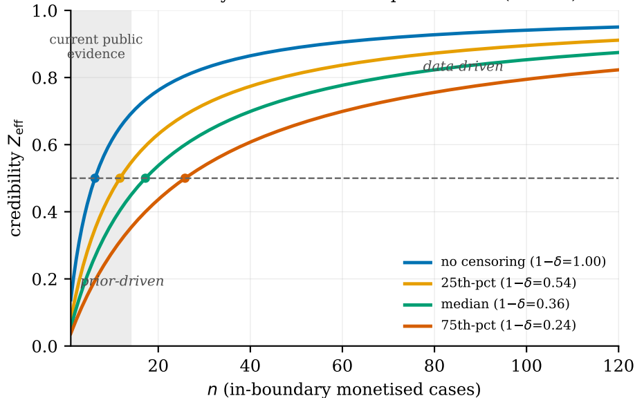
Identifiability frontier: data- vs prior-driven ( Z = 0.5 )
