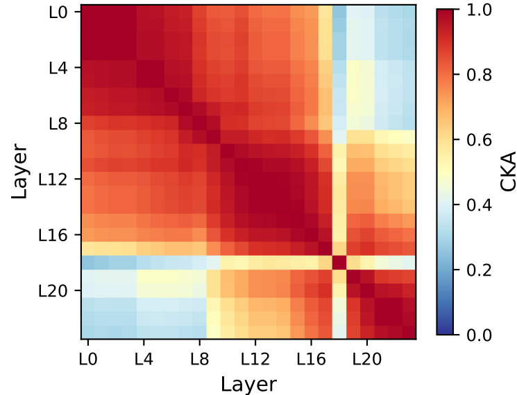
(A) Layer-wise CKA Matrix (Adult dataset)
