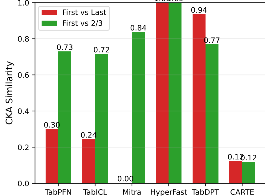
(C) Layer Similarity Summary
