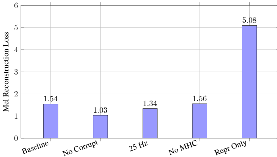
Figure 6: Visual comparison of the Mel-spectrogram Reconstruction Loss at 25,000 steps. Disabling reconstruction grounding (Repr Only) results in catastrophic acoustic loss, while removing decoder corruption (No Corrupt) artificially depresses the loss at the risk of overfitting.
