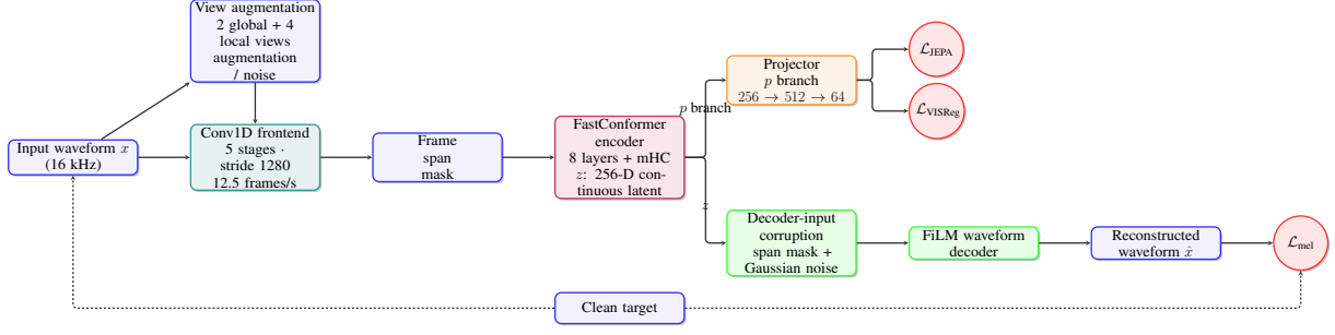
Figure 2: Detailed architecture of the Continuous Latent Autoencoder (CLAE). The clean input provides the reconstruction target. Augmented views pass through the frontend, frame masking, and encoder before branching into the representation ( p ) and waveform-reconstruction ( z ) objectives.
