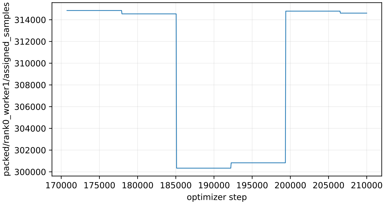
Pretraining segment 4
