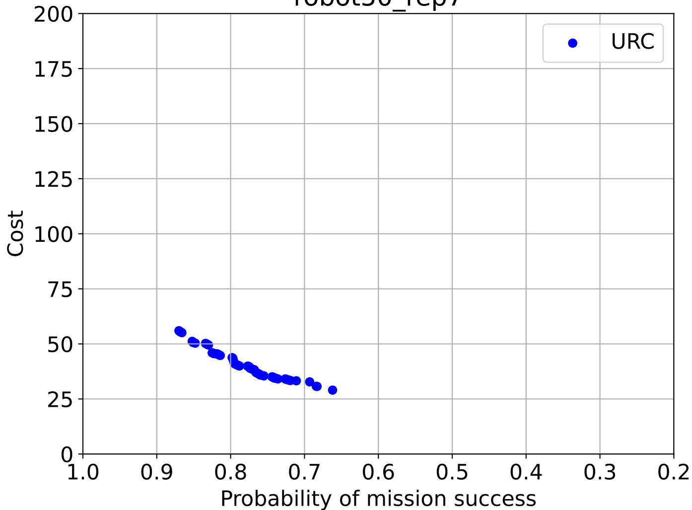
robot50_rep7
