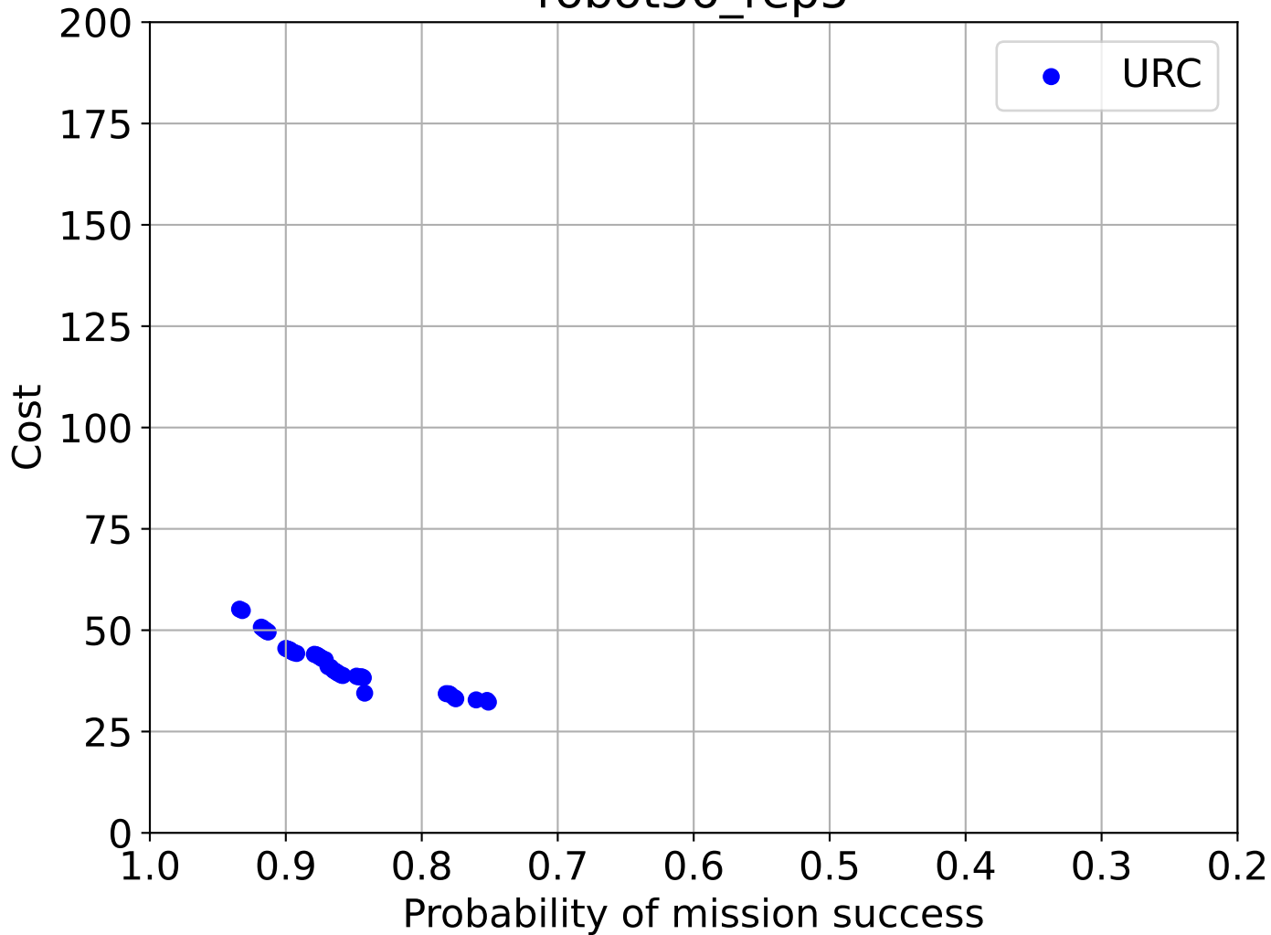
robot56_rep5
