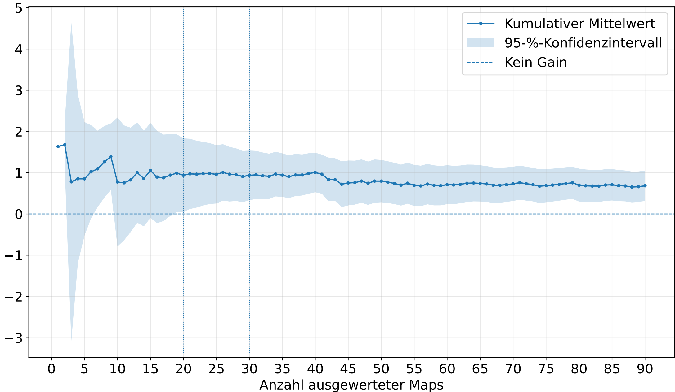
Mittlerer Hypervolume-Gain
