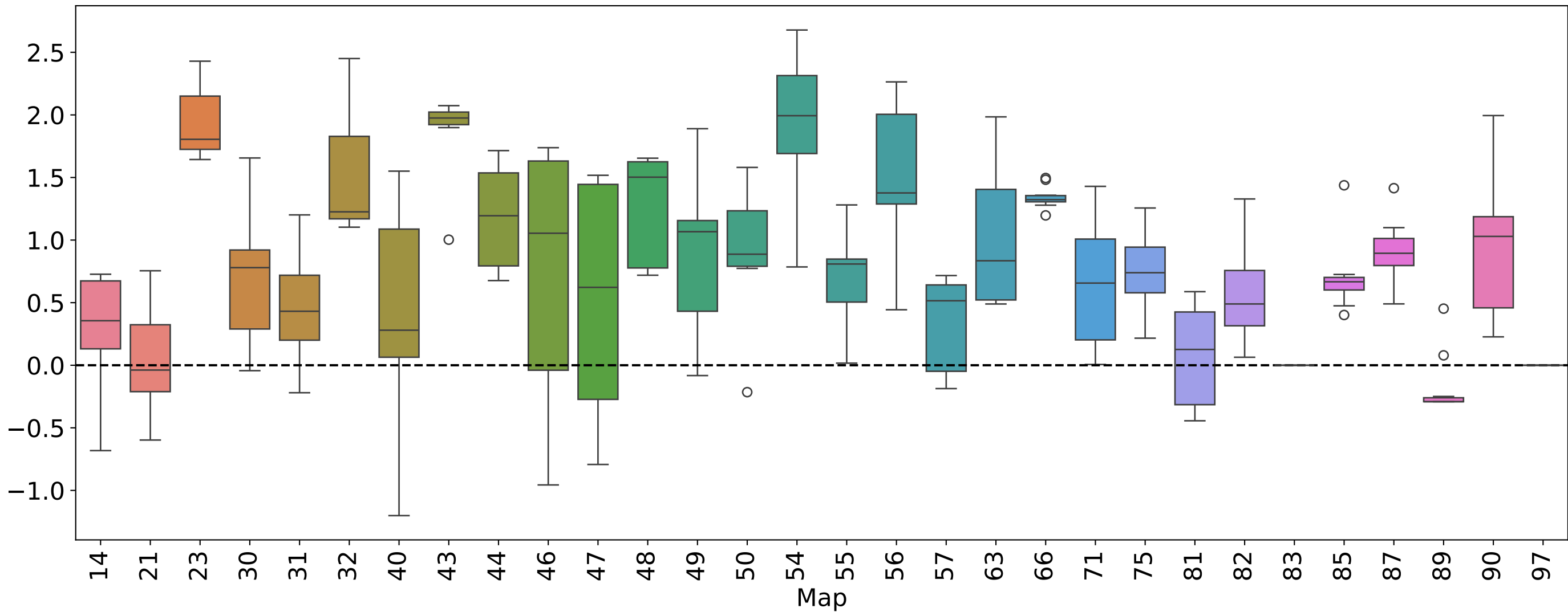
Hypervolume-Gains
