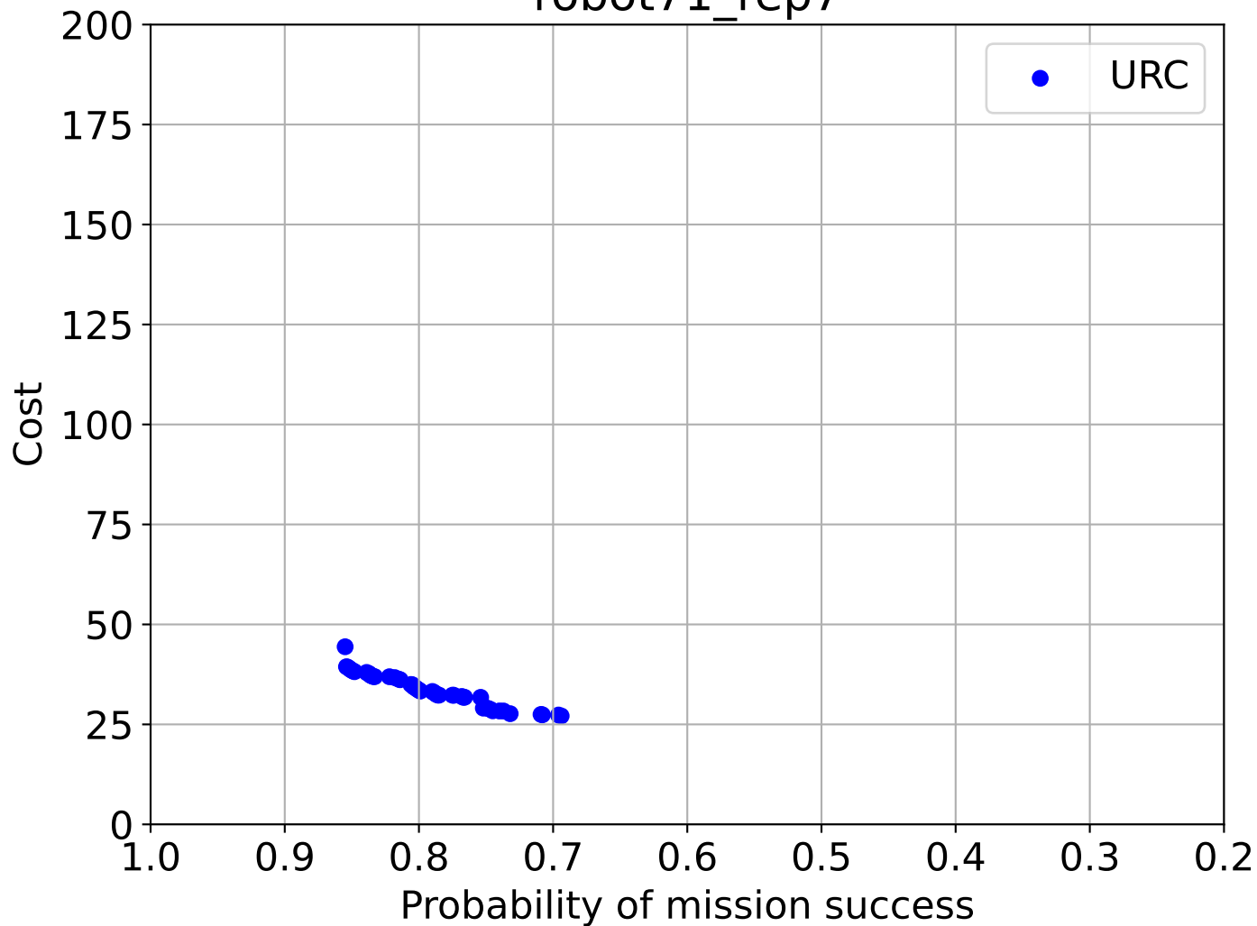
robot71_rep7
