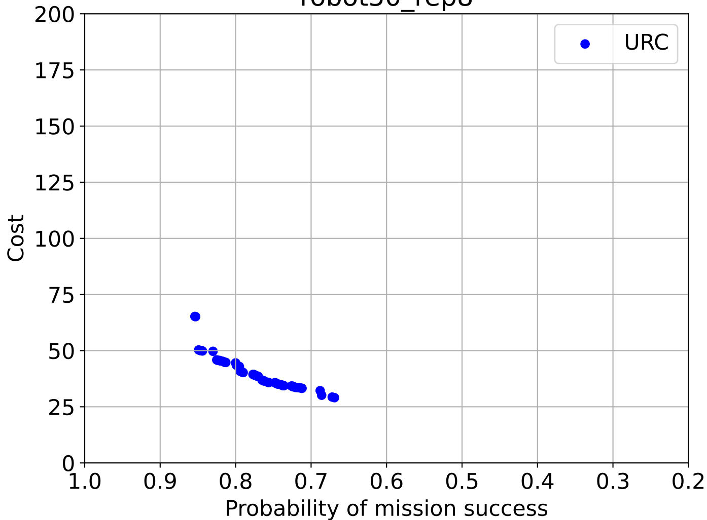
robot50_rep8
