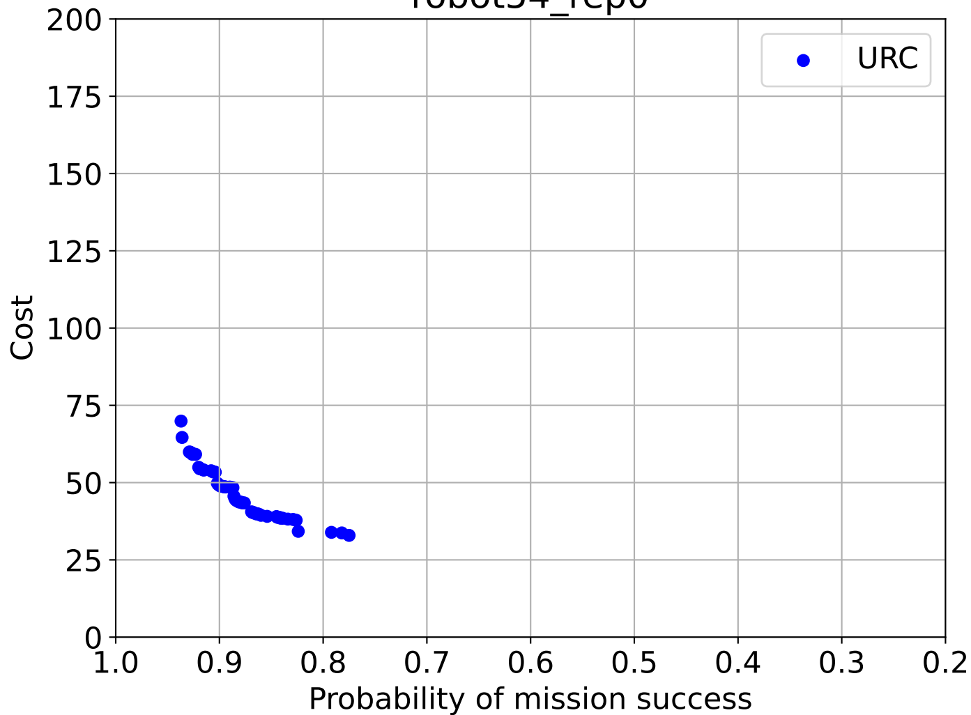
robot54_rep0
