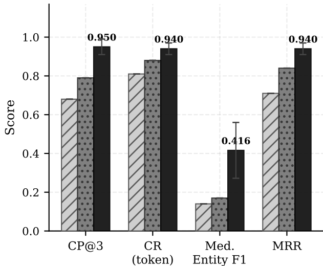
(a) Medical — PubMedQA
