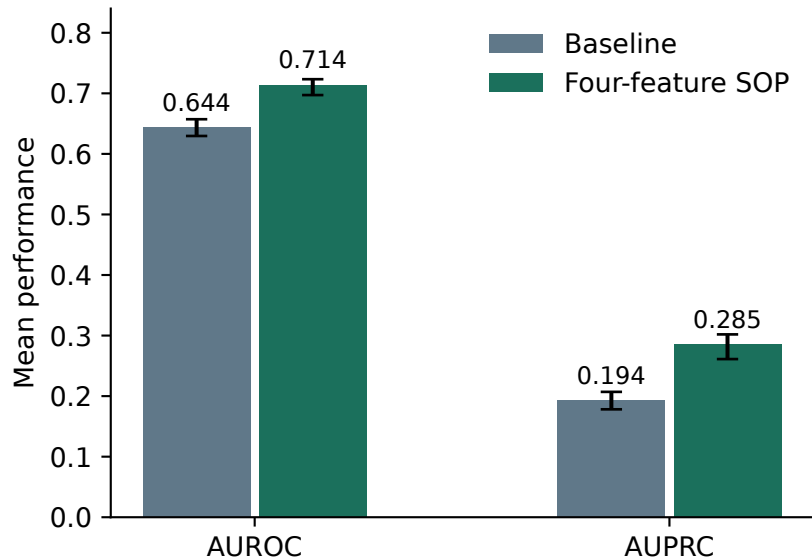
A Random-order prediction comparison
