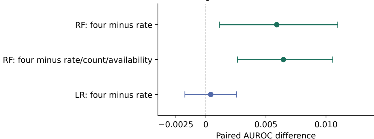
B Residual gain from four features
