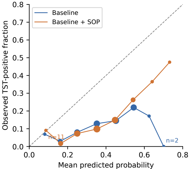
A Uncalibrated scores
