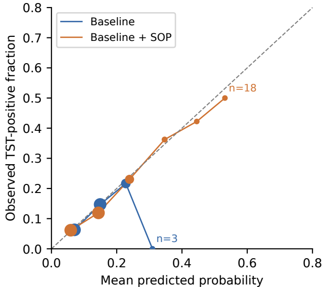
B Nested calibration
