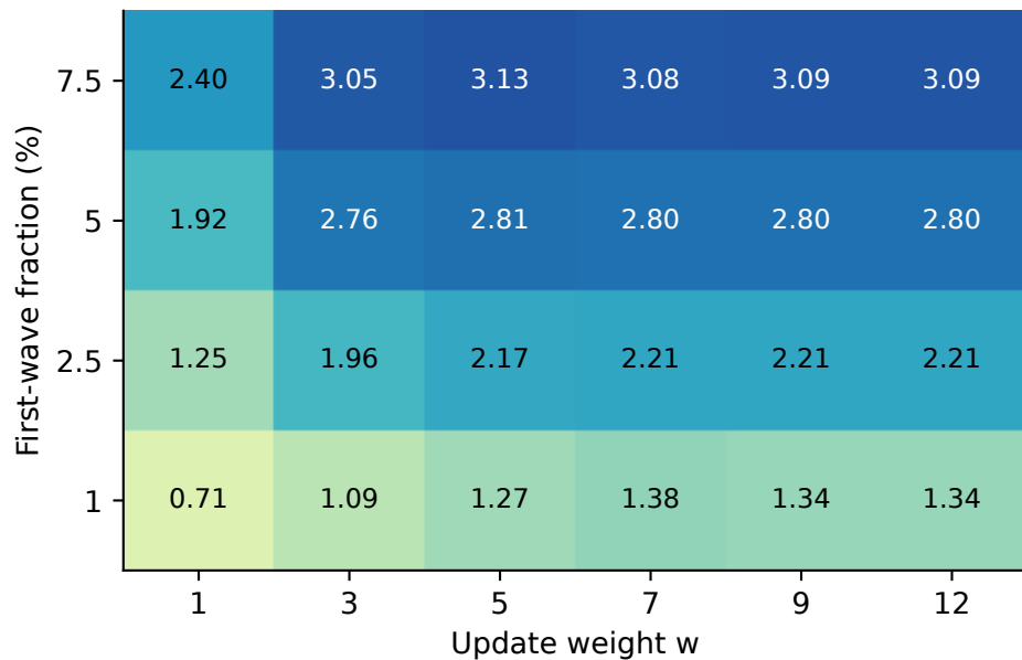
RF: capture difference (percentage points)
