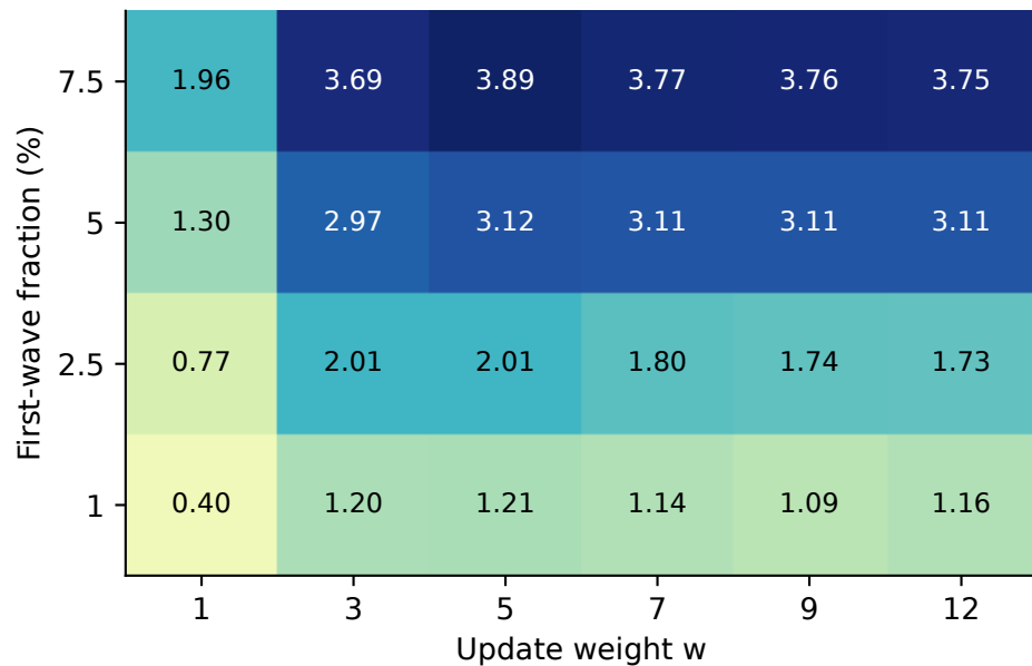
LR: capture difference (percentage points)
