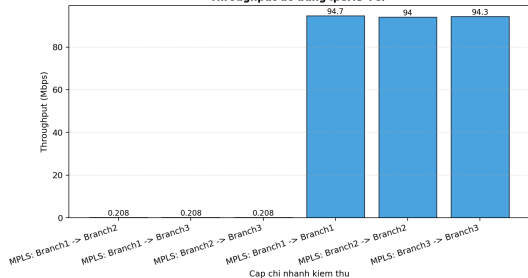
Throughput do bang iperf3 TCP
