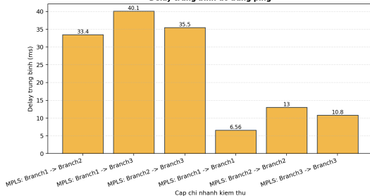
Delay trung bình do bang ping
