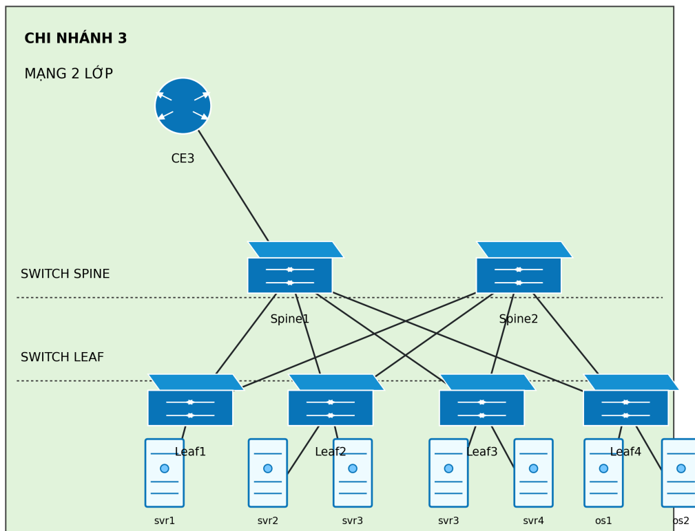
Hình 3.4 Branch 3 Leaf-Spine Network
