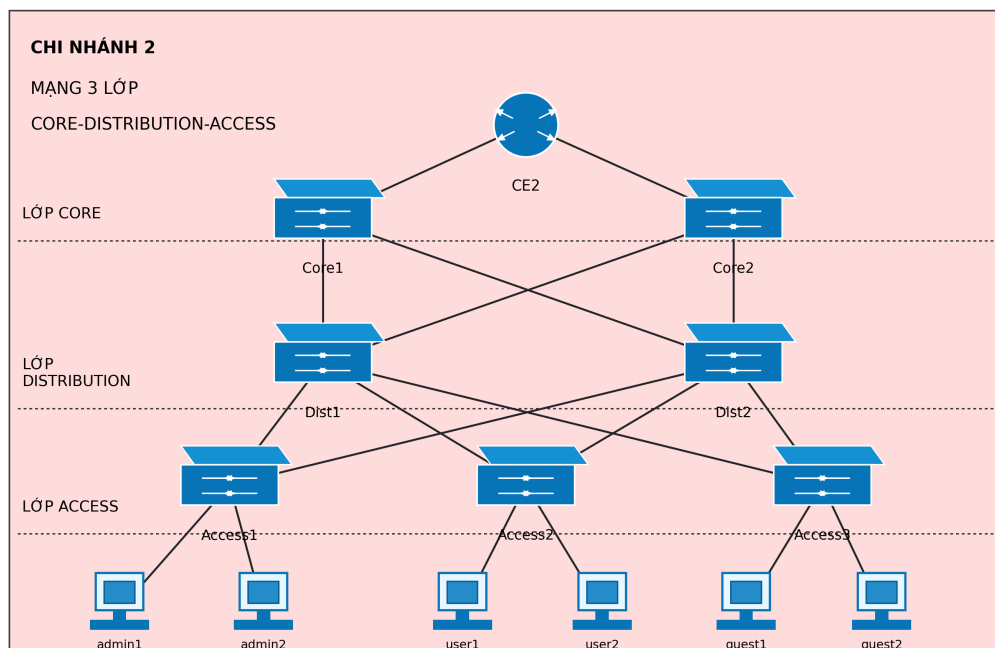
Hình 3.3 Branch 2 Three-tier Network
