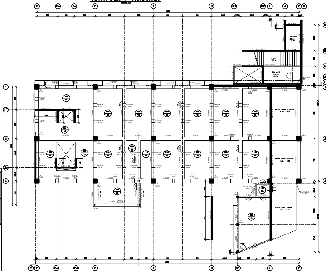
(LOSA c=15 (S.I.C.)) (NIVEL SUPERIOR LOSA -0.05) PLANTA CIELO PISO 1° Escala 1:50
