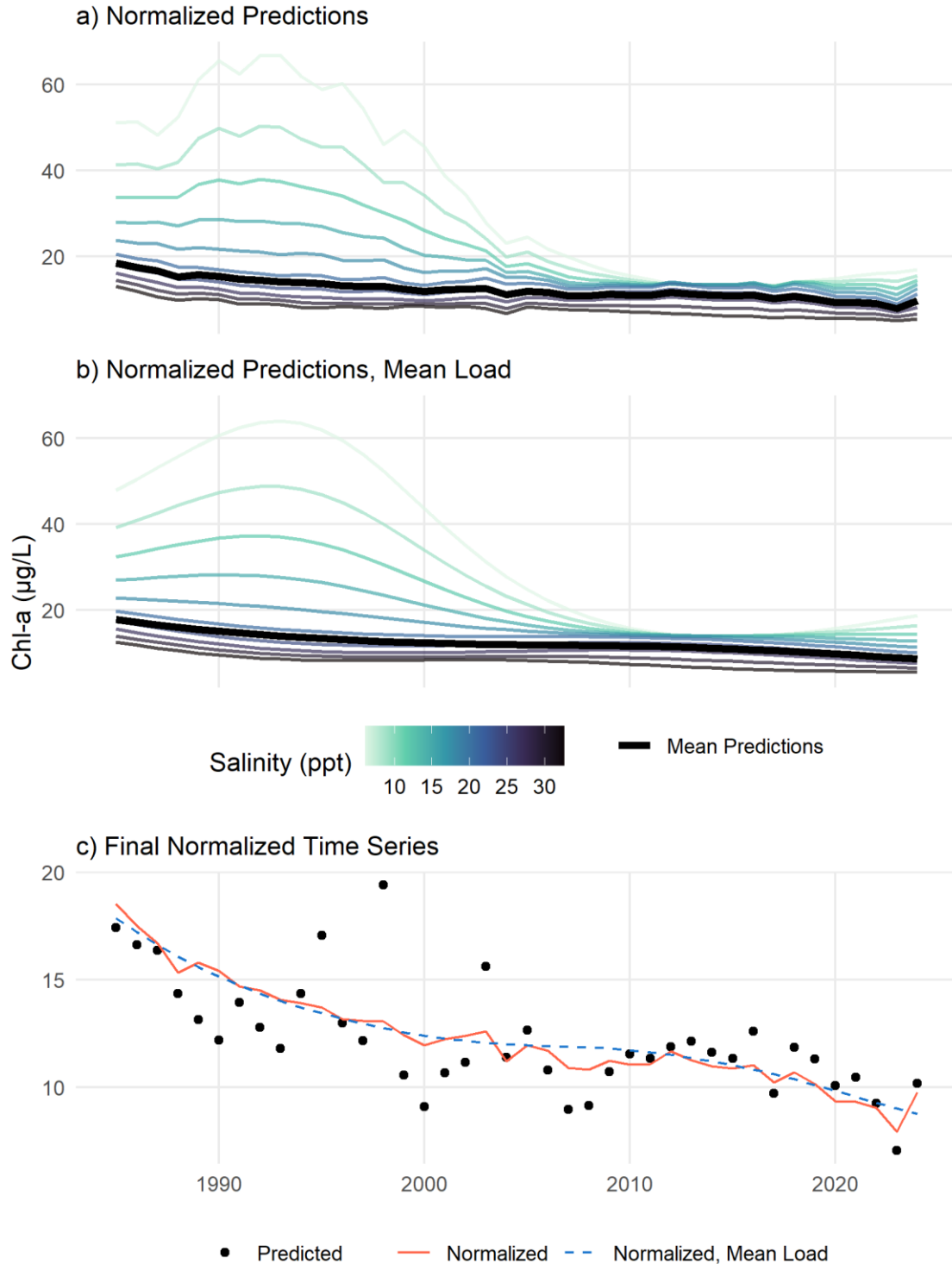
Fig. 1: Examples demonstrating the salinity normalization method (a), the salinity normalization method at mean loading (b), and the final results (c). Results are obtained by predicting chlorophyll-a concentrations from a fitted GAM across a range of salinities and estimating the
