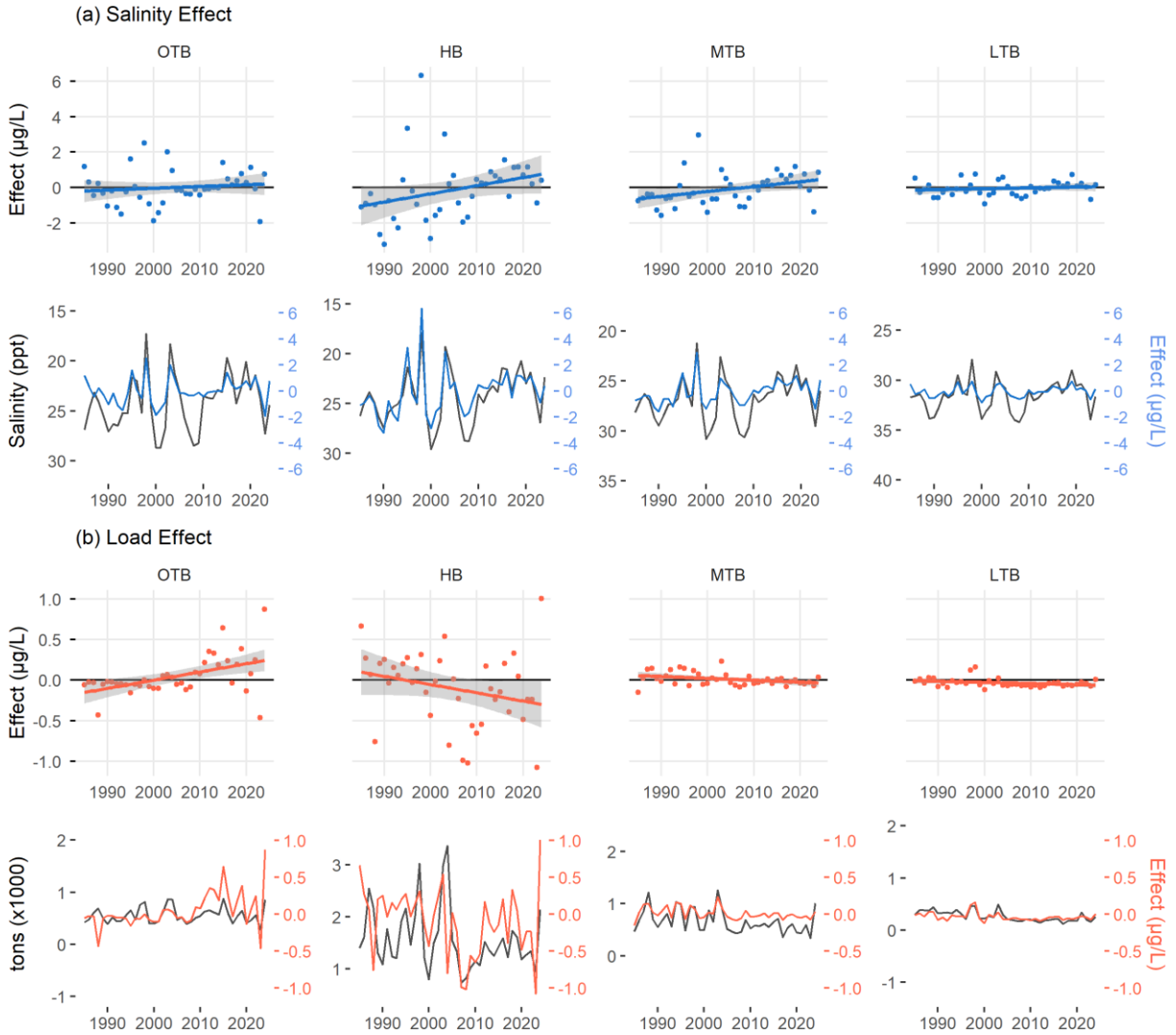
Fig. 5: Unique effects of salinity (a) and loading (b) on chlorophyll-a concentrations over time by bay segment. Points in the first and third rows represent values for a given year where the model predictions minus the salinity-normalized results show the effect of salinity (a) and the salinity-normalized results minus the normalized results at mean loading show the effect of loading (b). Linear trends and standard errors across years are also shown. Plots in rows two and four show the same values for the salinity or loading effects as in rows one and three on the right axes, but with the actual salinity and loading values included on the left axes. Note that the salinity axis in row two is reversed. OTB: Old Tampa Bay; HB: Hillsborough Bay; MTB: Middle Tampa Bay; LTB: Lower Tampa Bay.
