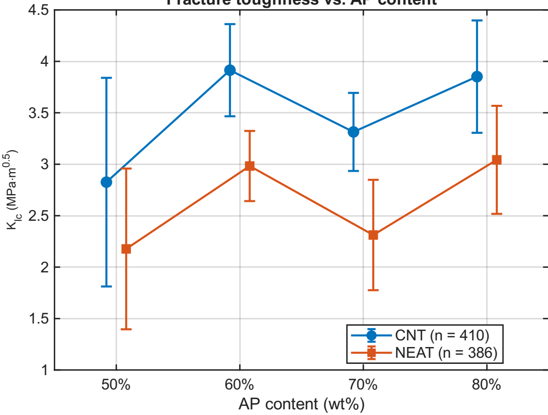
Fracture toughness vs. AP content
