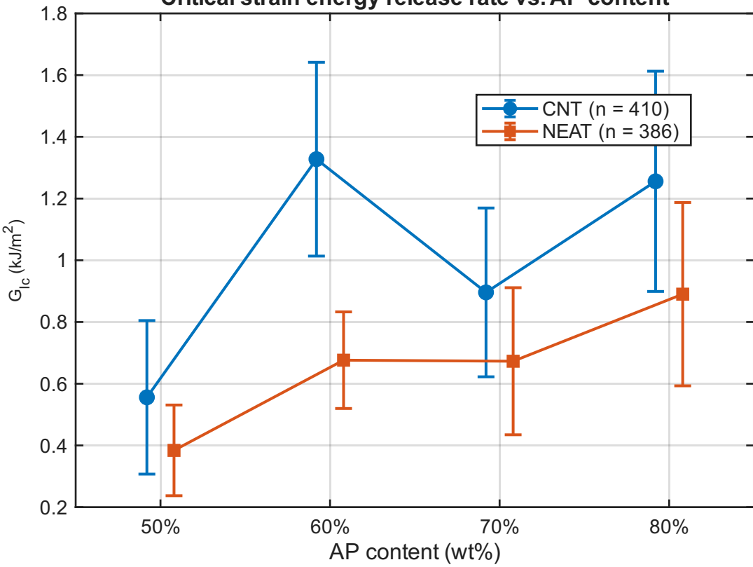
Critical strain energy release rate vs. AP content
