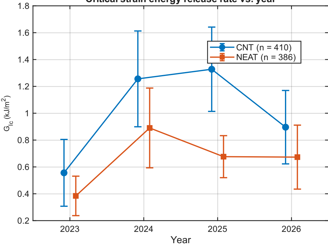
Critical strain energy release rate vs. year
