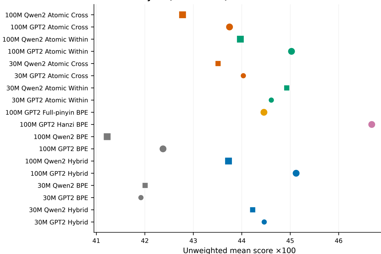
Official BabyLM (n=16 tasks)
