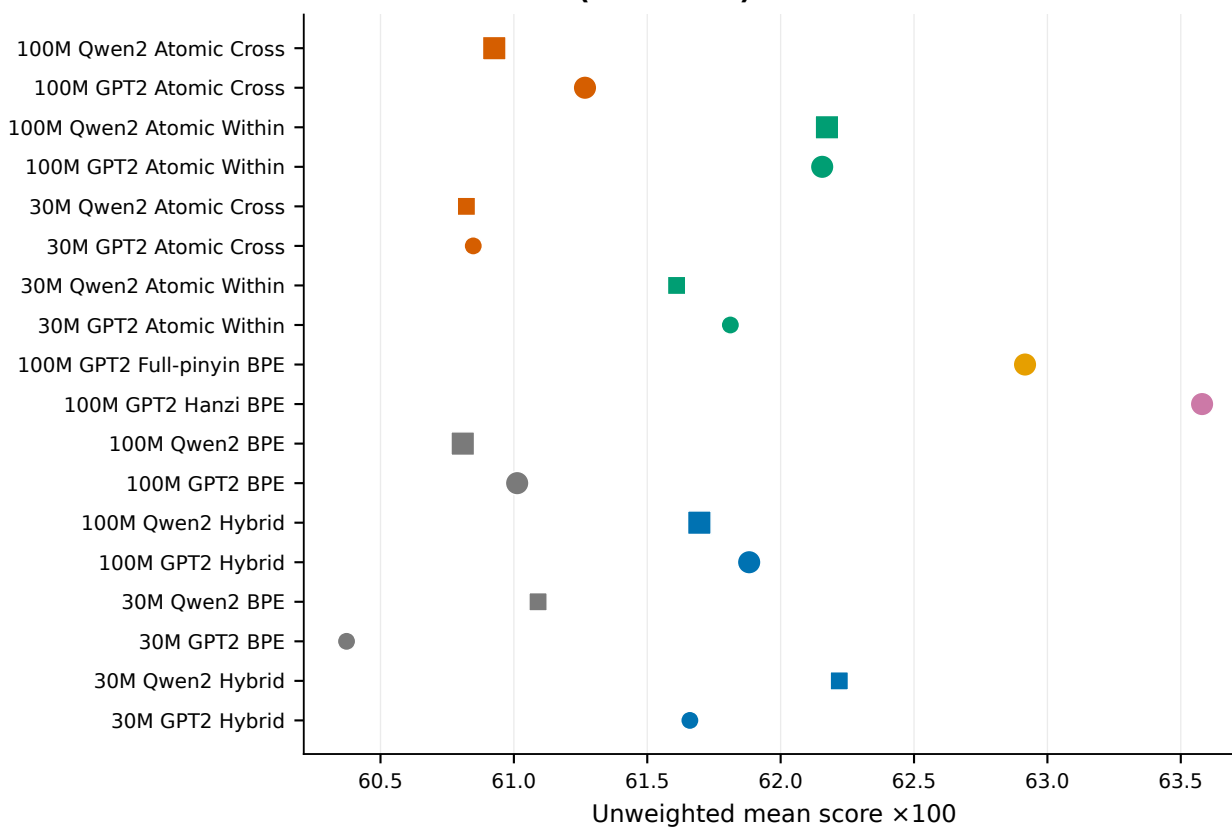
Chinese fine-tune (n=4 tasks)
