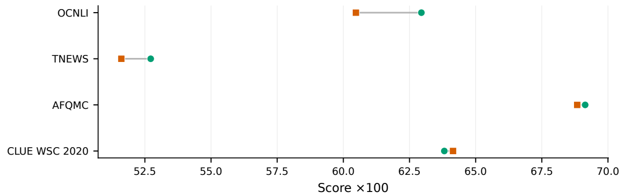
E Chinese fine-tune — GPT2
