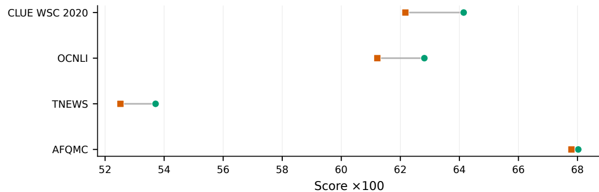
F Chinese fine-tune — Qwen2
