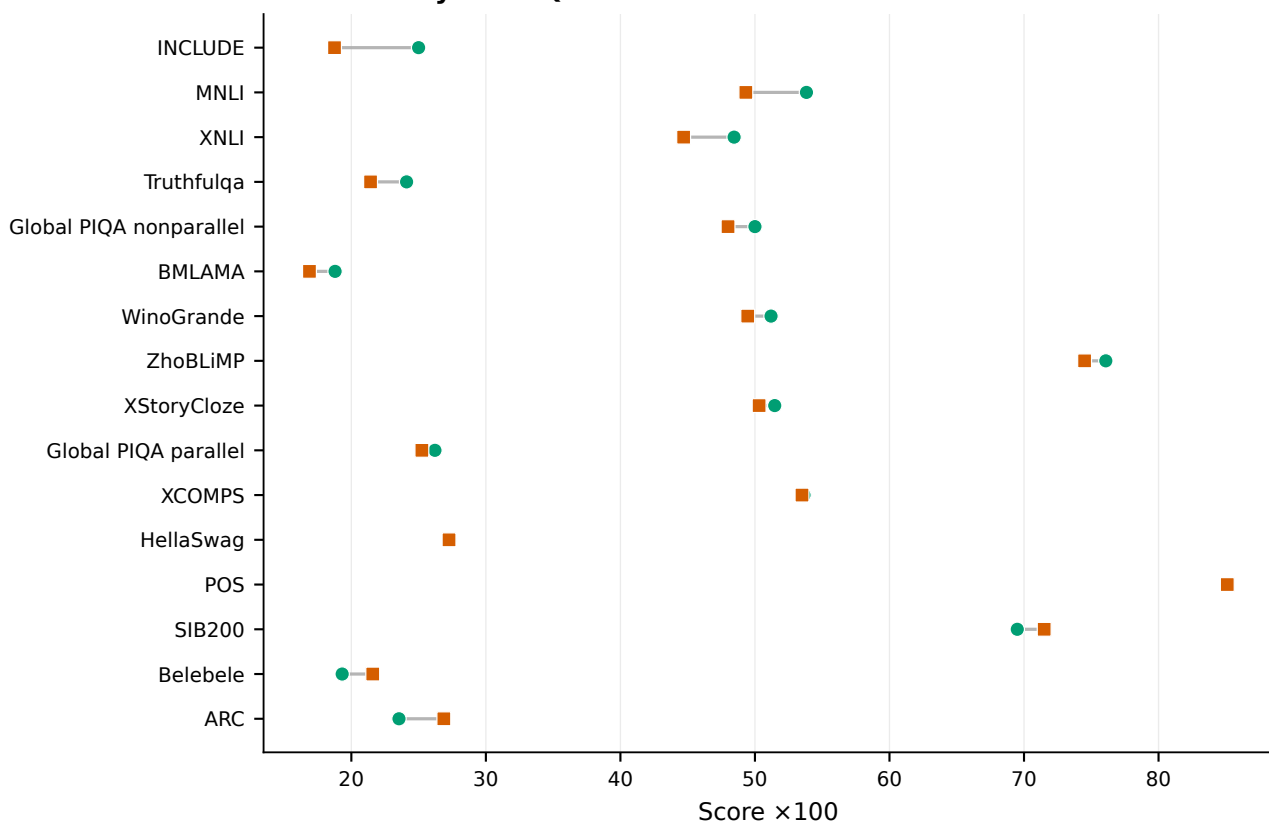
B Official BabyLM — Qwen2
