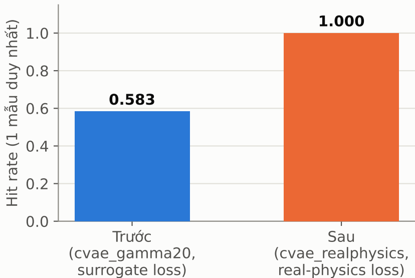
Hit rate single-shot — trước/sau fix surrogate-exploitation
