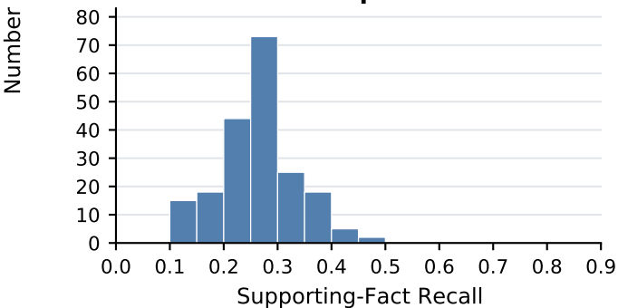
16x compression
