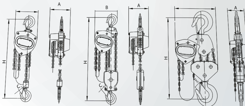
EPC - 0.5T TO 2T
