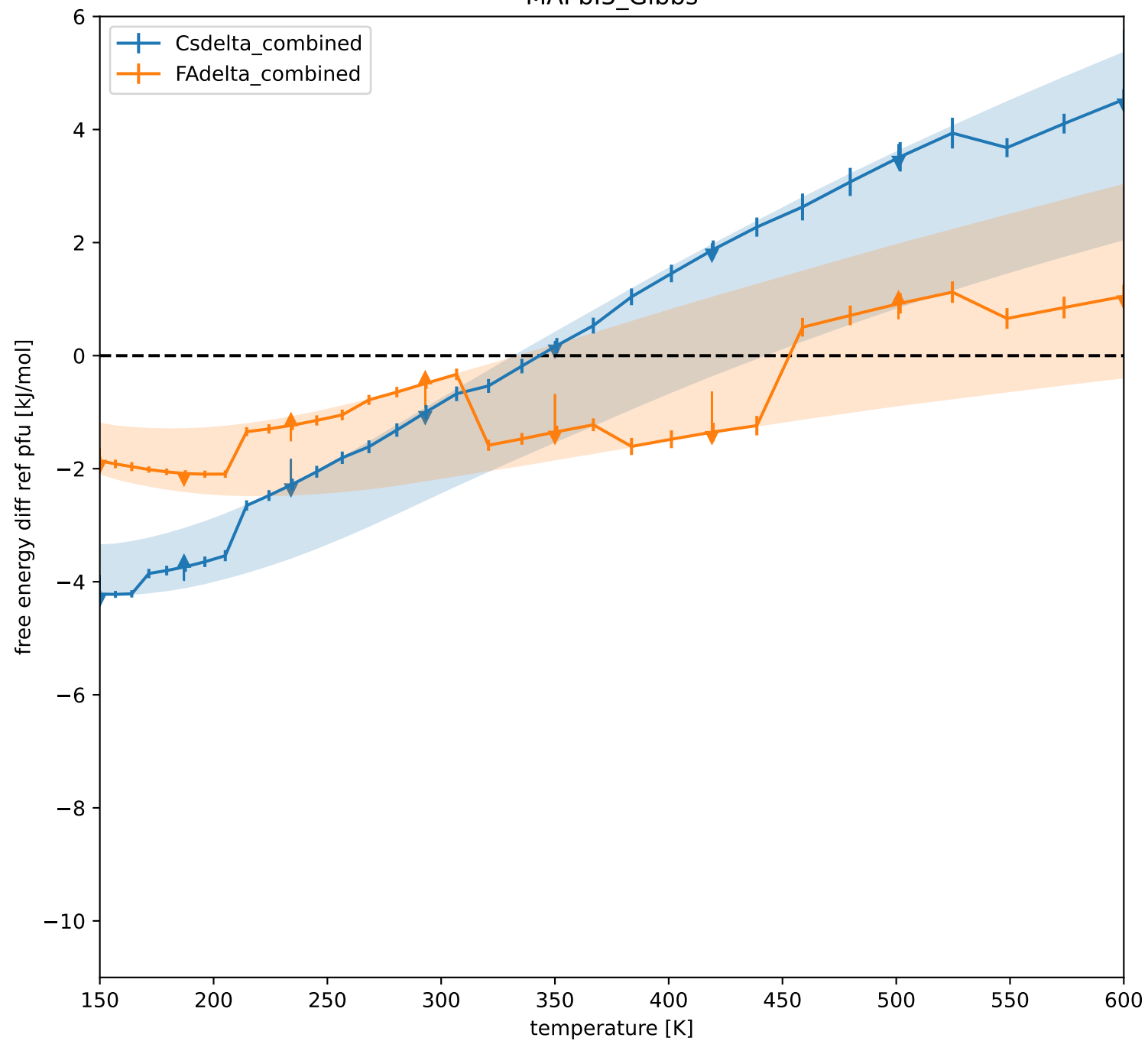
MAPbI3_Gibbs
