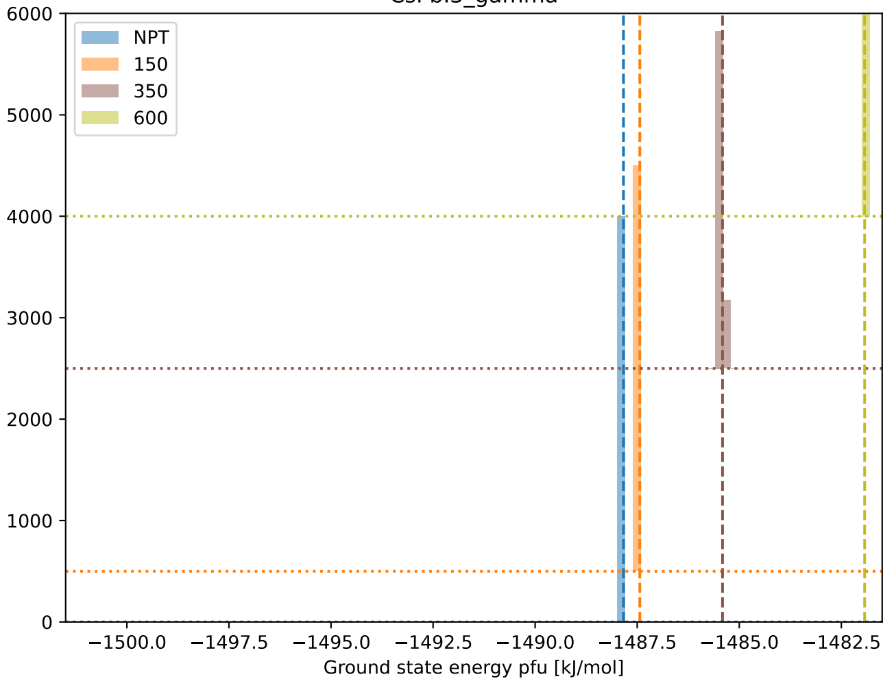
CsPbI3_gamma
