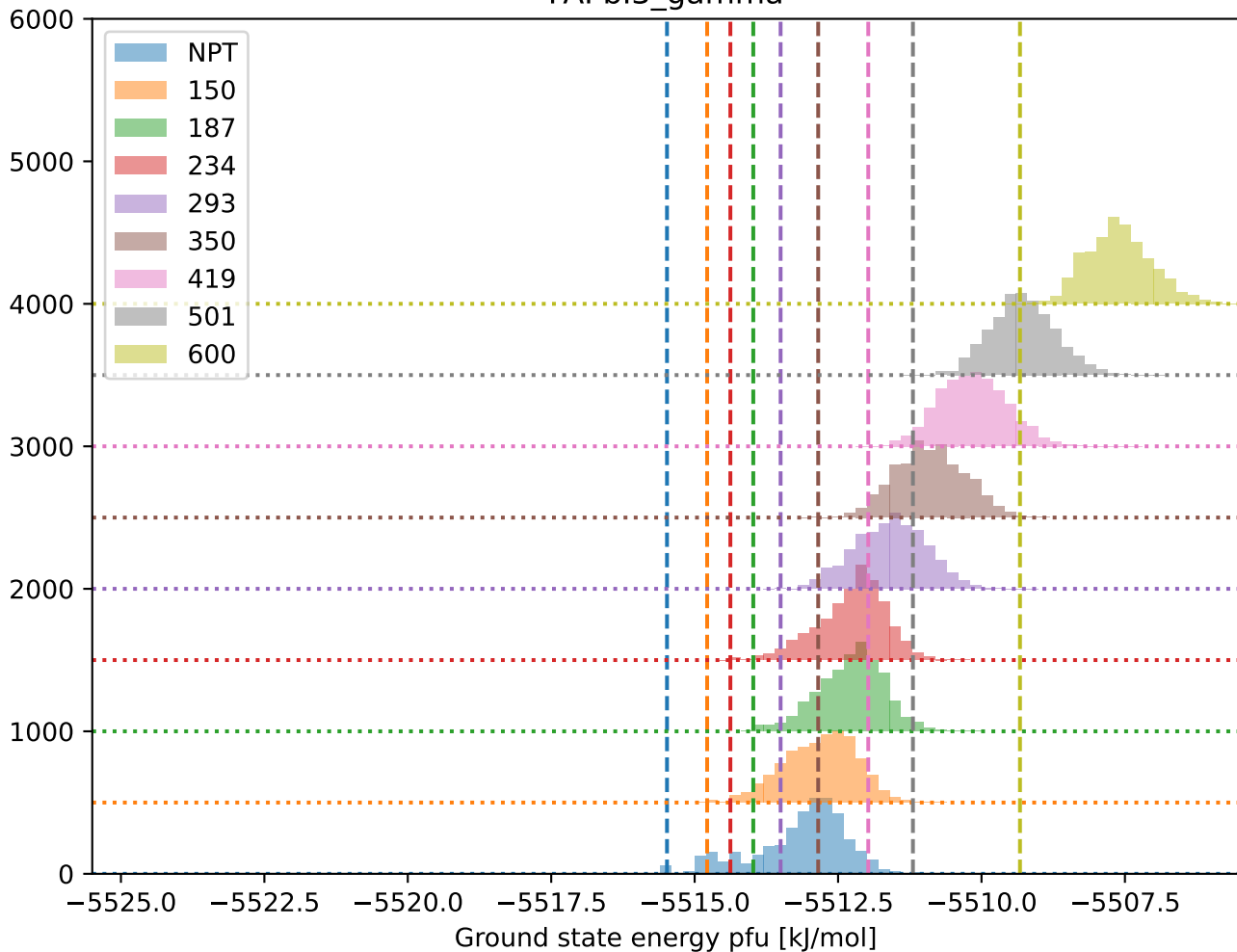
FAPbI3_gamma
