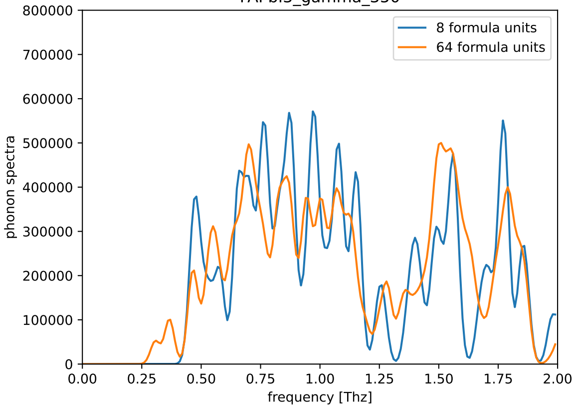
FAPbI3_gamma_350
