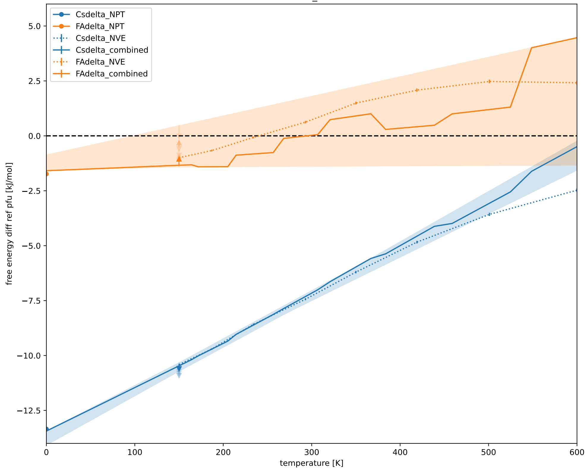
CsPbI3_Harm
