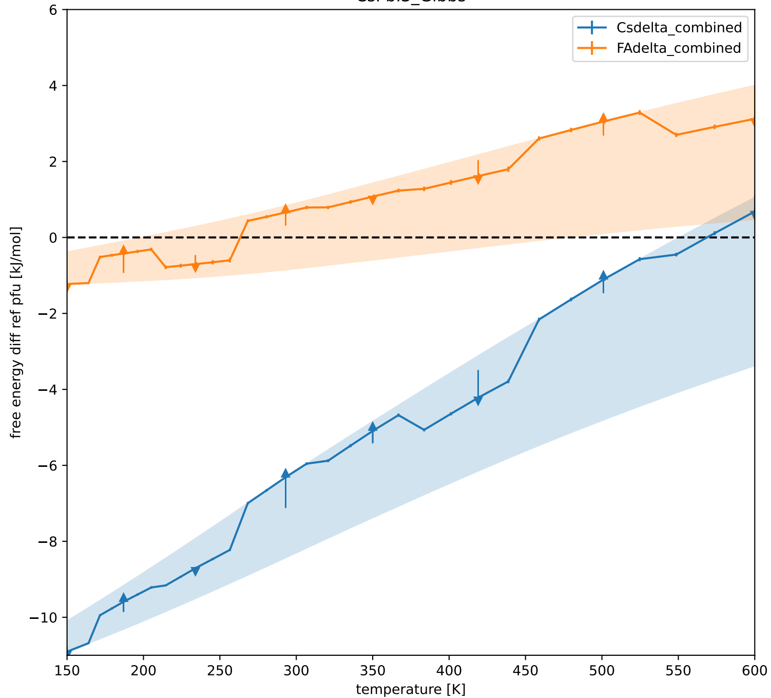
CsPbI3_Gibbs
