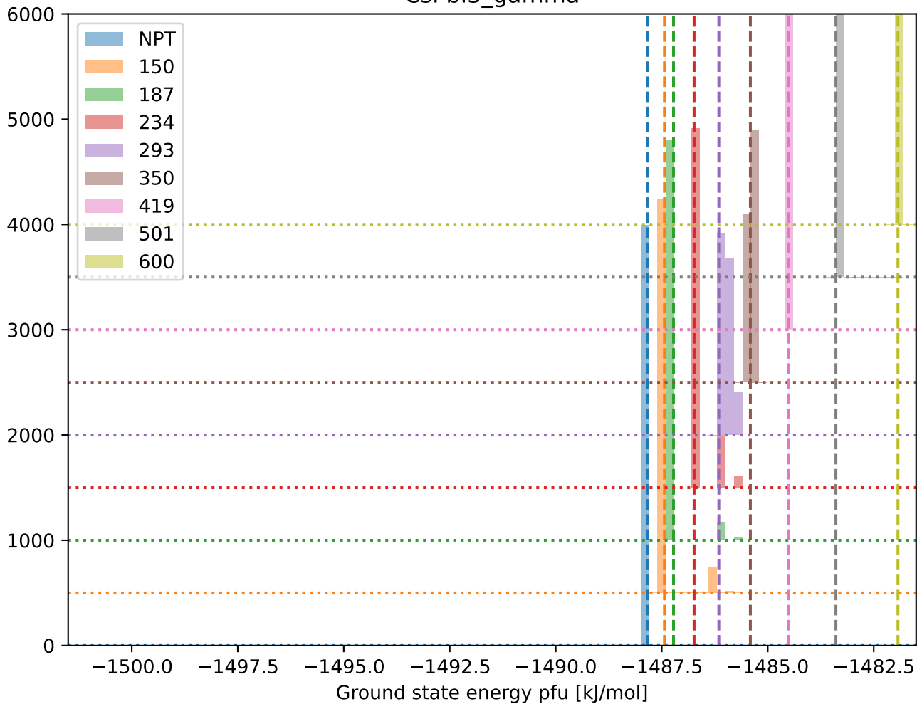
CsPbI3_gamma
