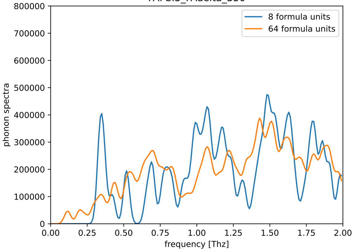
FAPbI3_FAdelta_350
