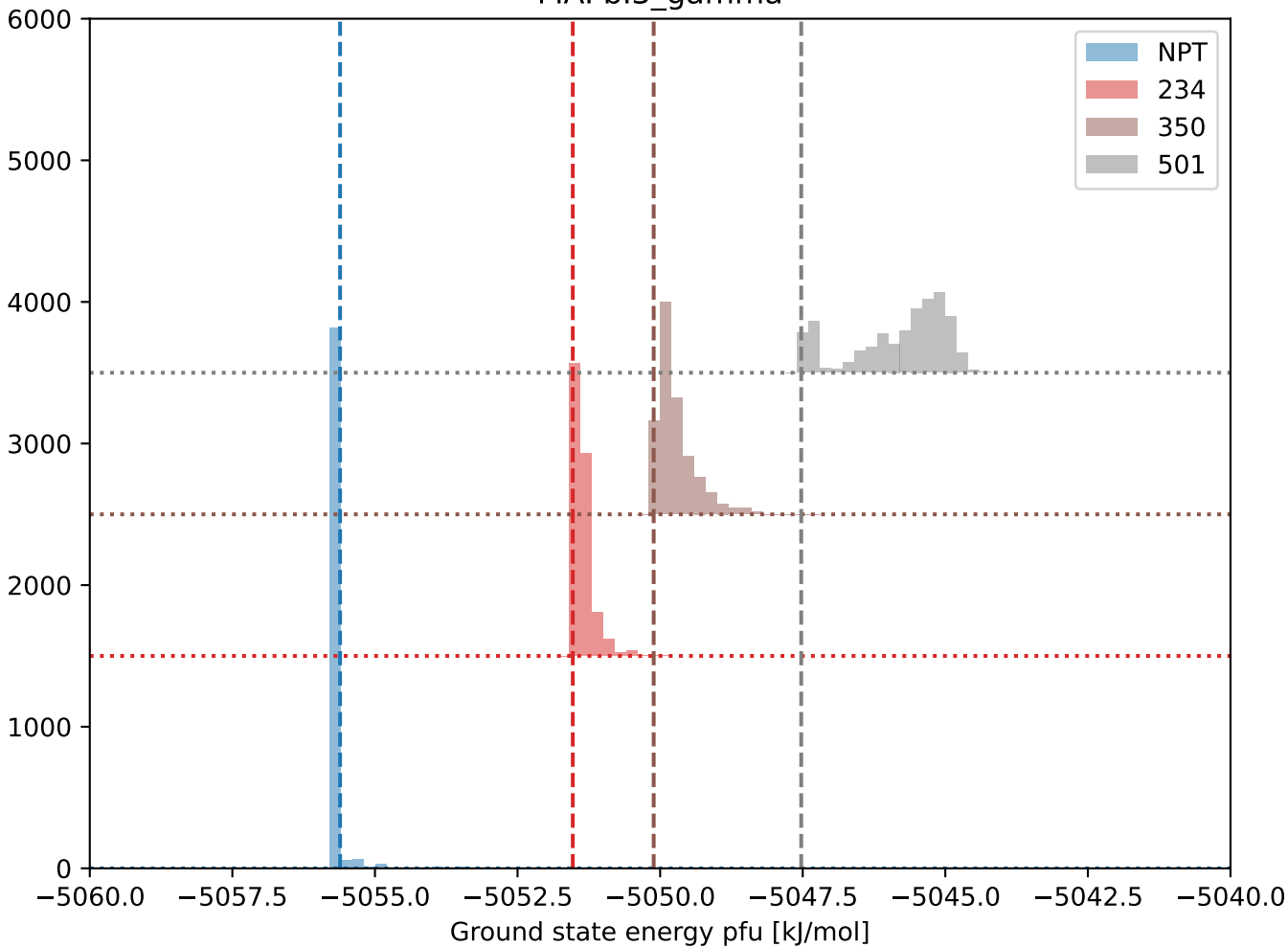
MAPbI3_gamma
