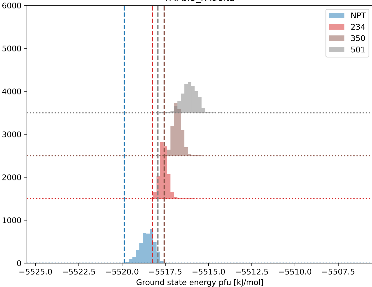
FAPbI3_FAdelta
