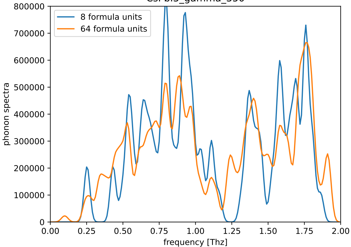
CsPbI3_gamma_350
