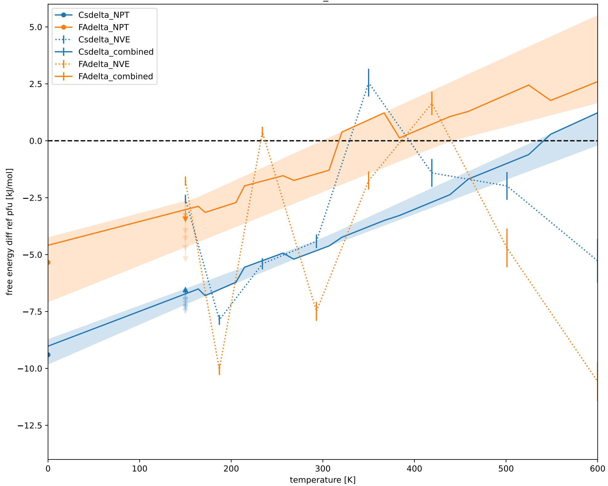
FAPbl3_Harm
