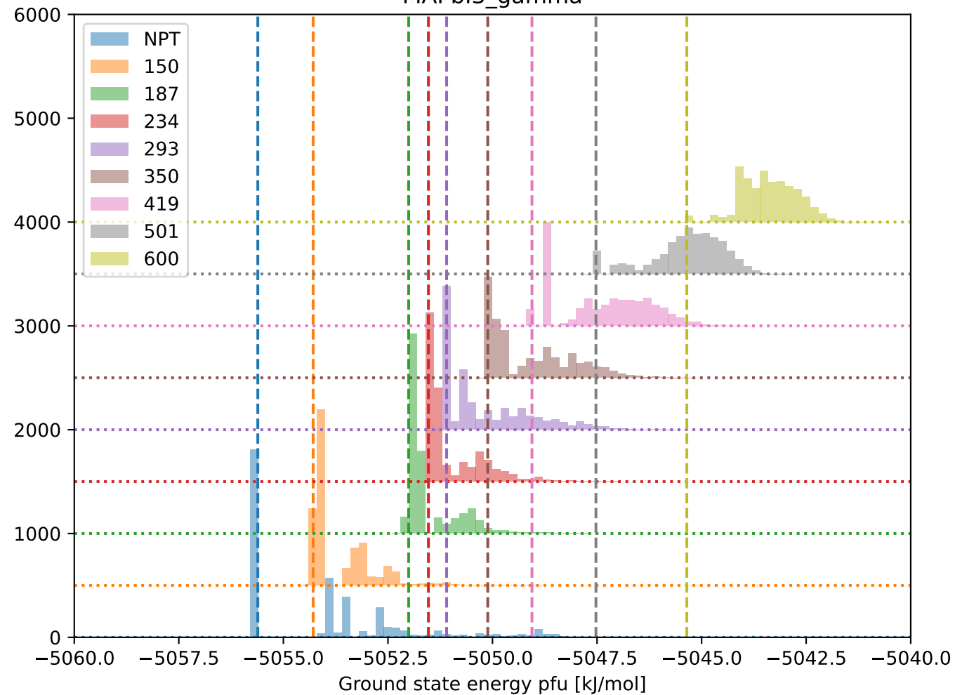
MAPbI3_gamma
