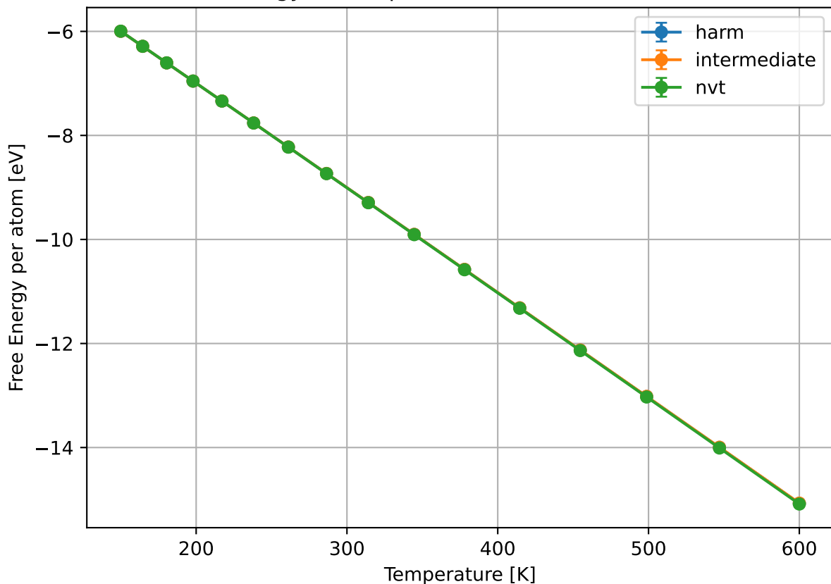
Free Energy vs Temperature with reference at 150K
