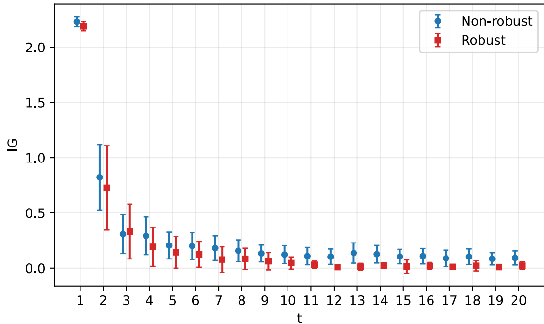
IG in \theta ( s = 3.00 )
