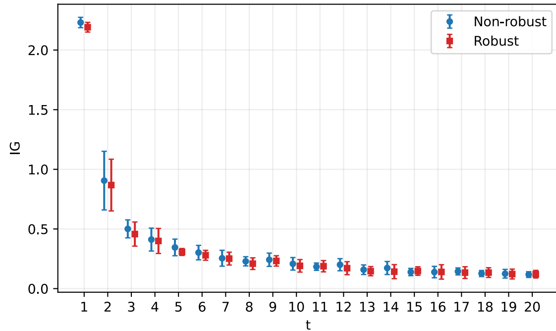
IG in \theta ( s = 1.00 )
