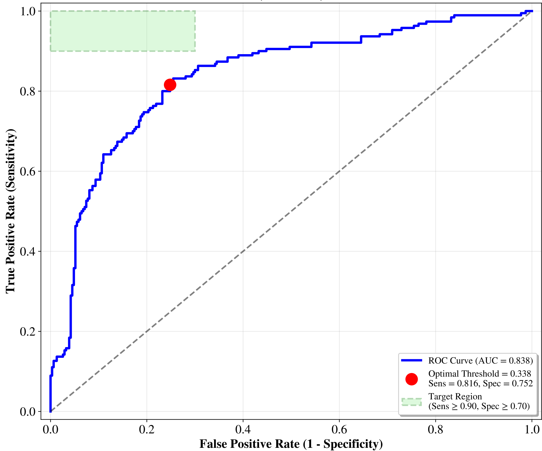
ROC Curve - HMV-MIL (TEST Set)
