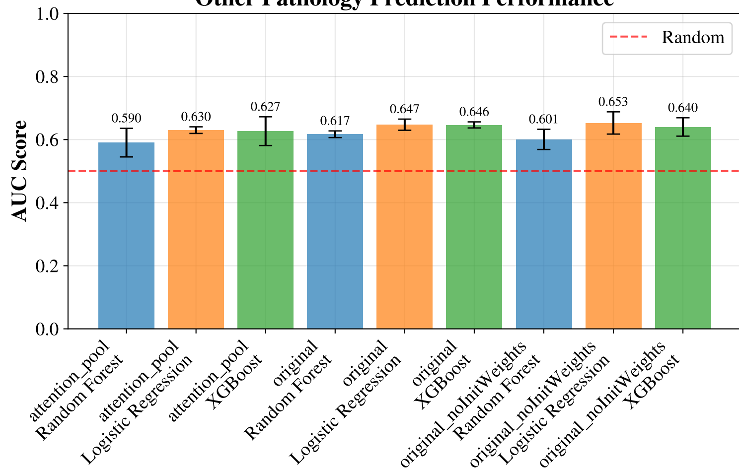
Model Configuration
