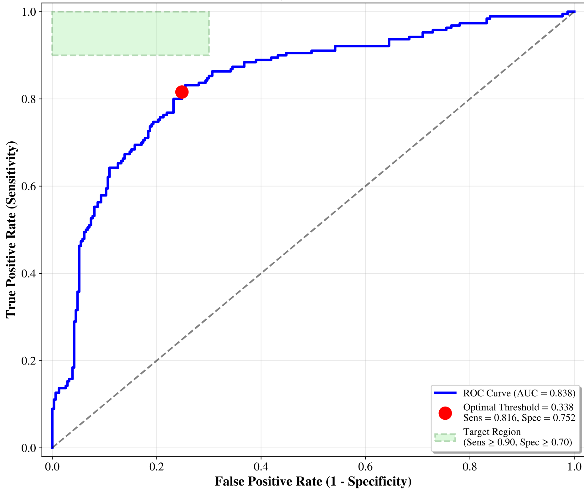
ROC Curve - HMV-MIL (TEST Set)
