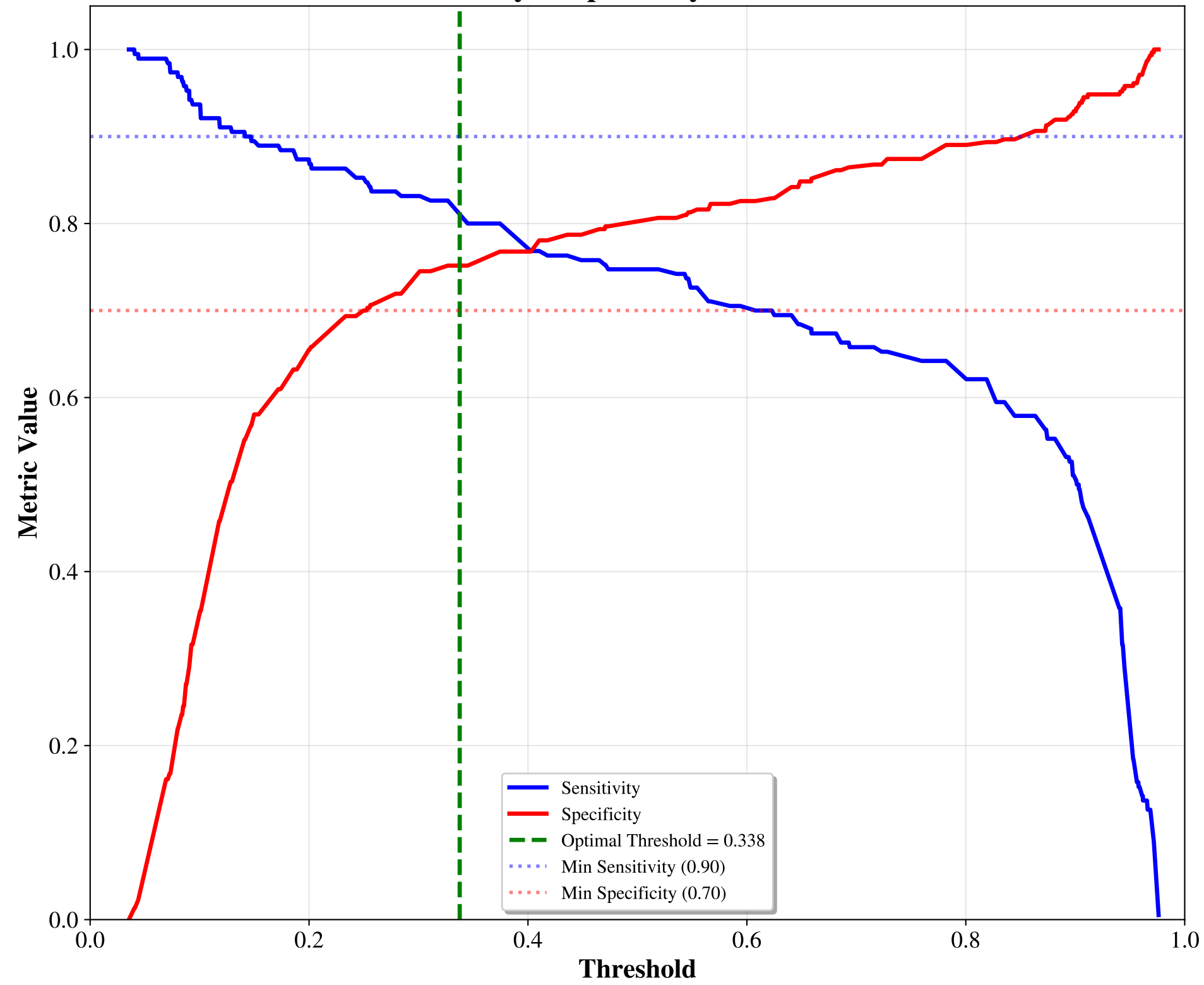
Sensitivity & Specificity vs Threshold
