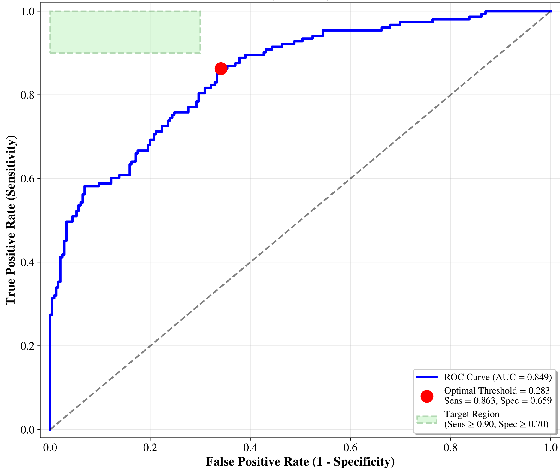
ROC Curve - Attention Pool Extra3 (VAL Set)
