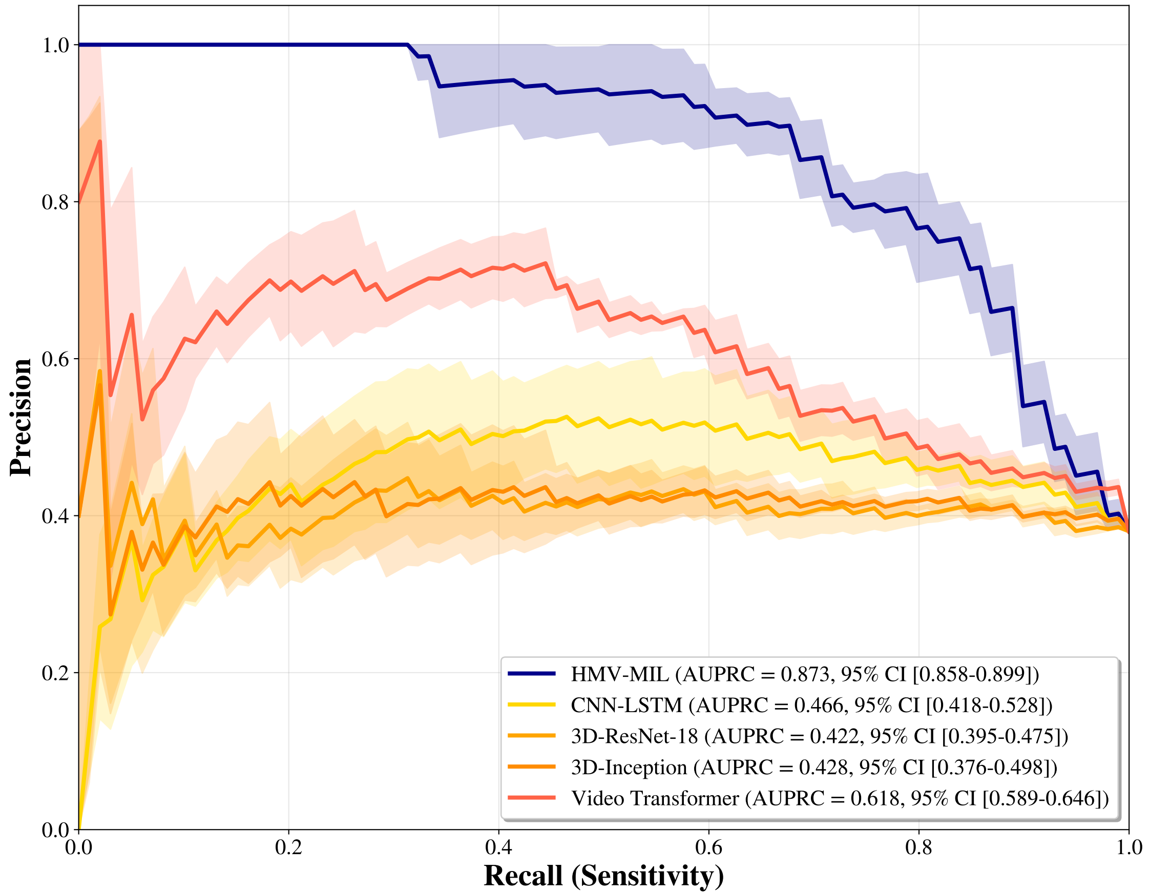
Precision-Recall Curves with 95% Confidence Intervals (Test Set)
