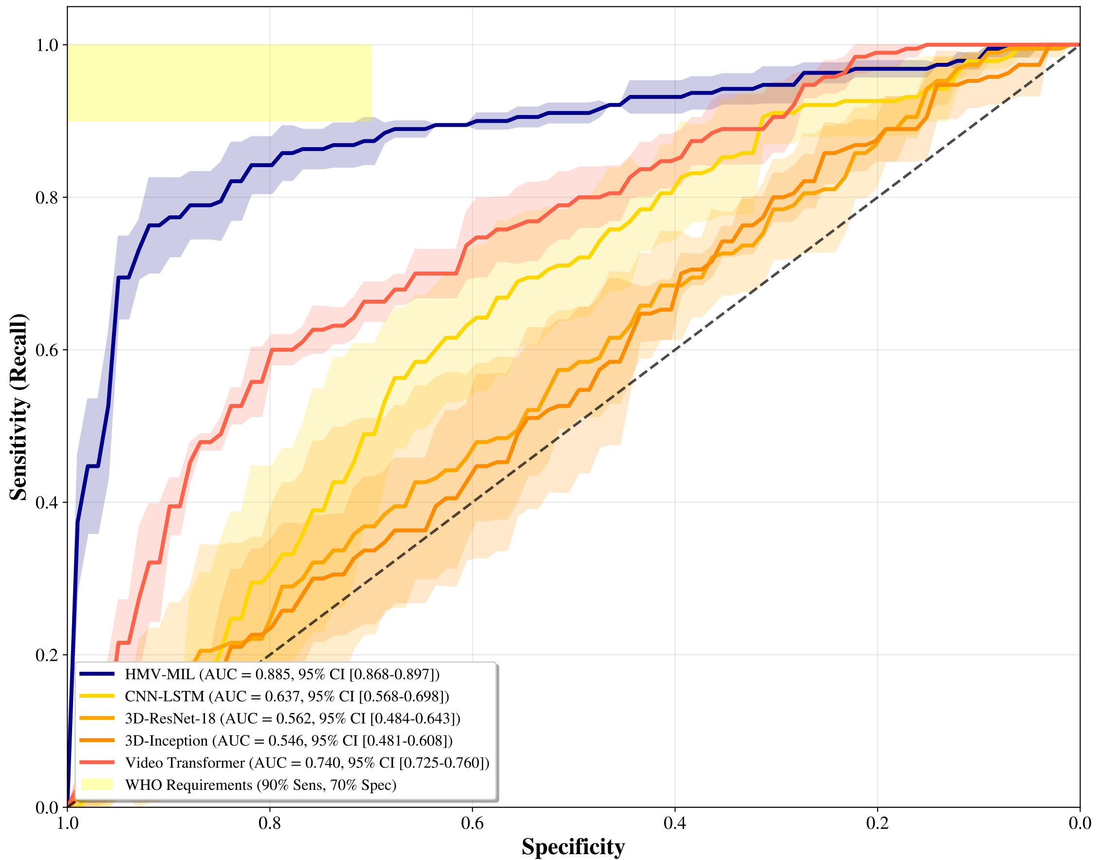
ROC Curves with 95% Confidence Intervals (Test Set) All Models
