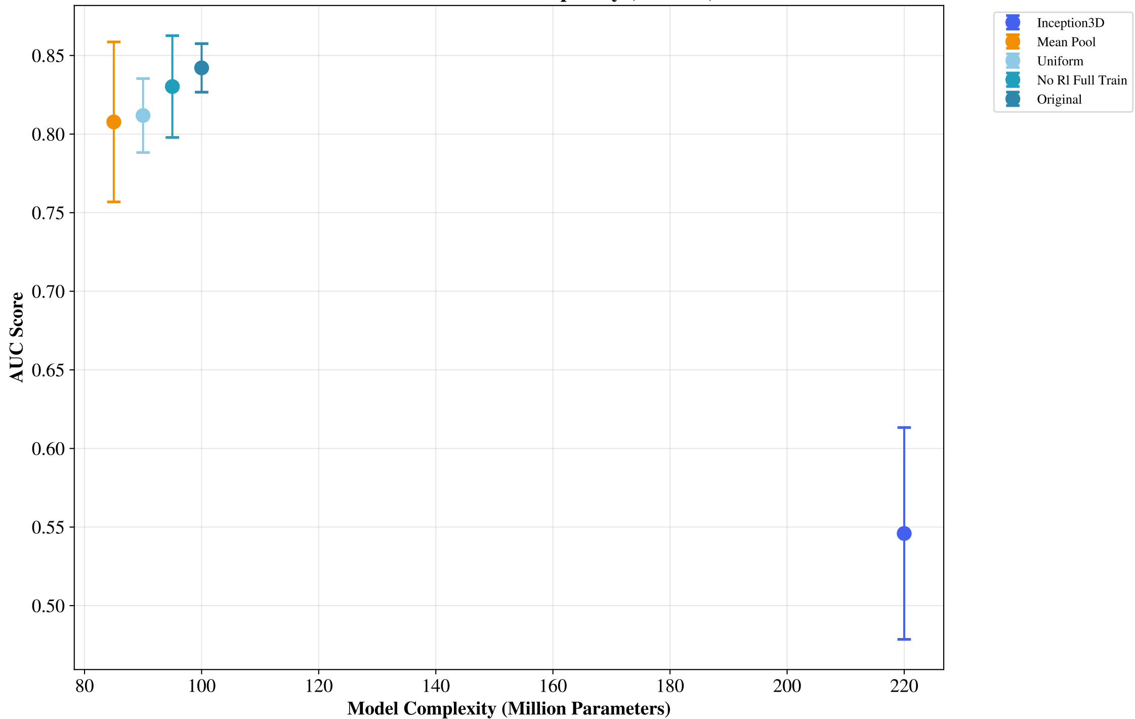
Performance vs Model Complexity (Test Set)
