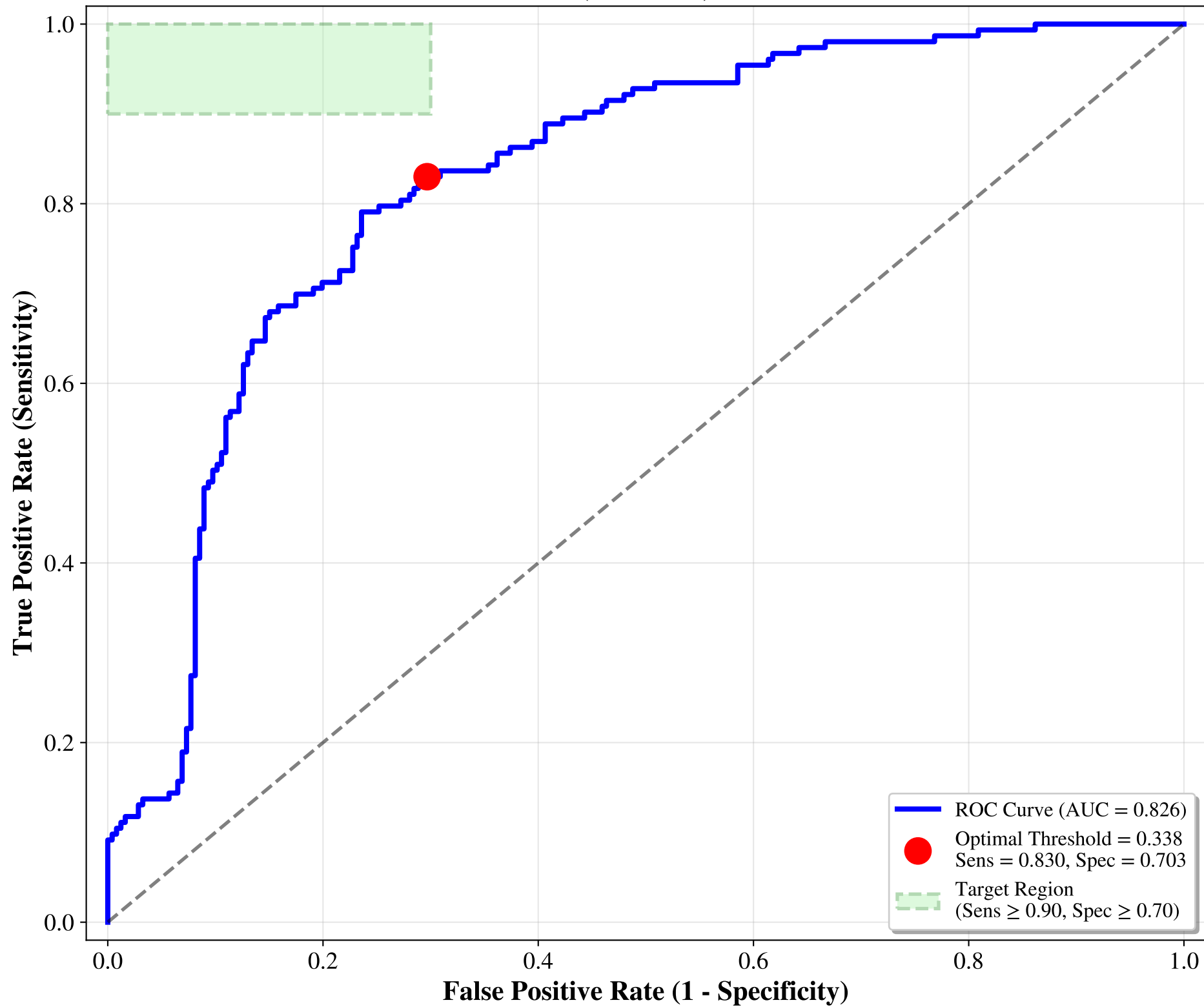
ROC Curve - HMV-MIL (VAL Set)
