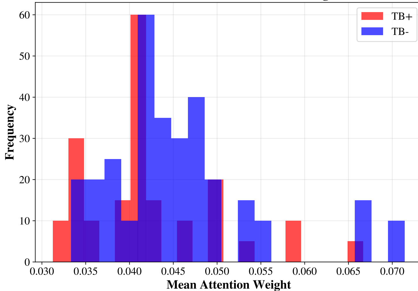
Distribution of Mean Attention Weights
