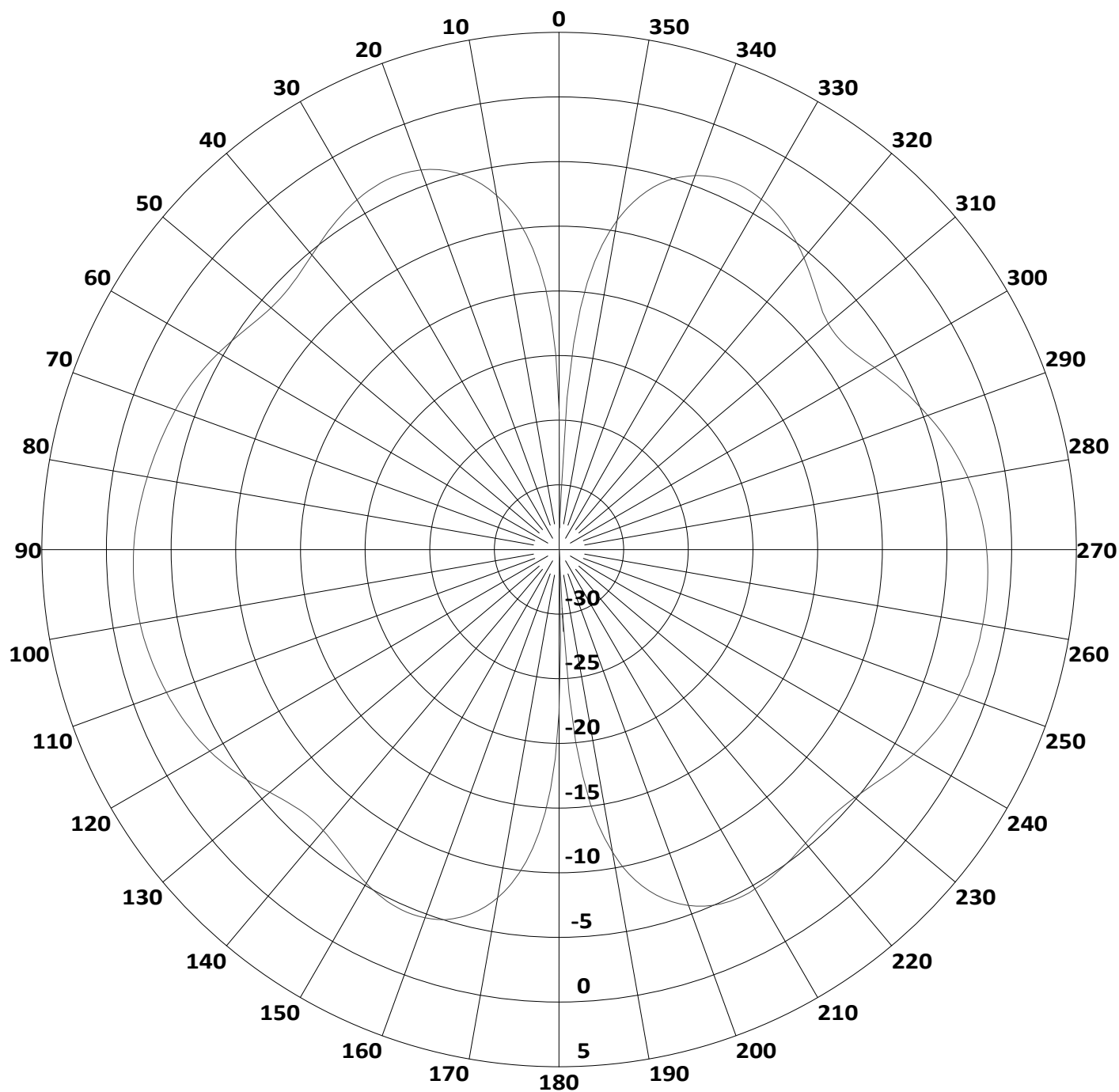
Gain (dBi) vs. Angle
